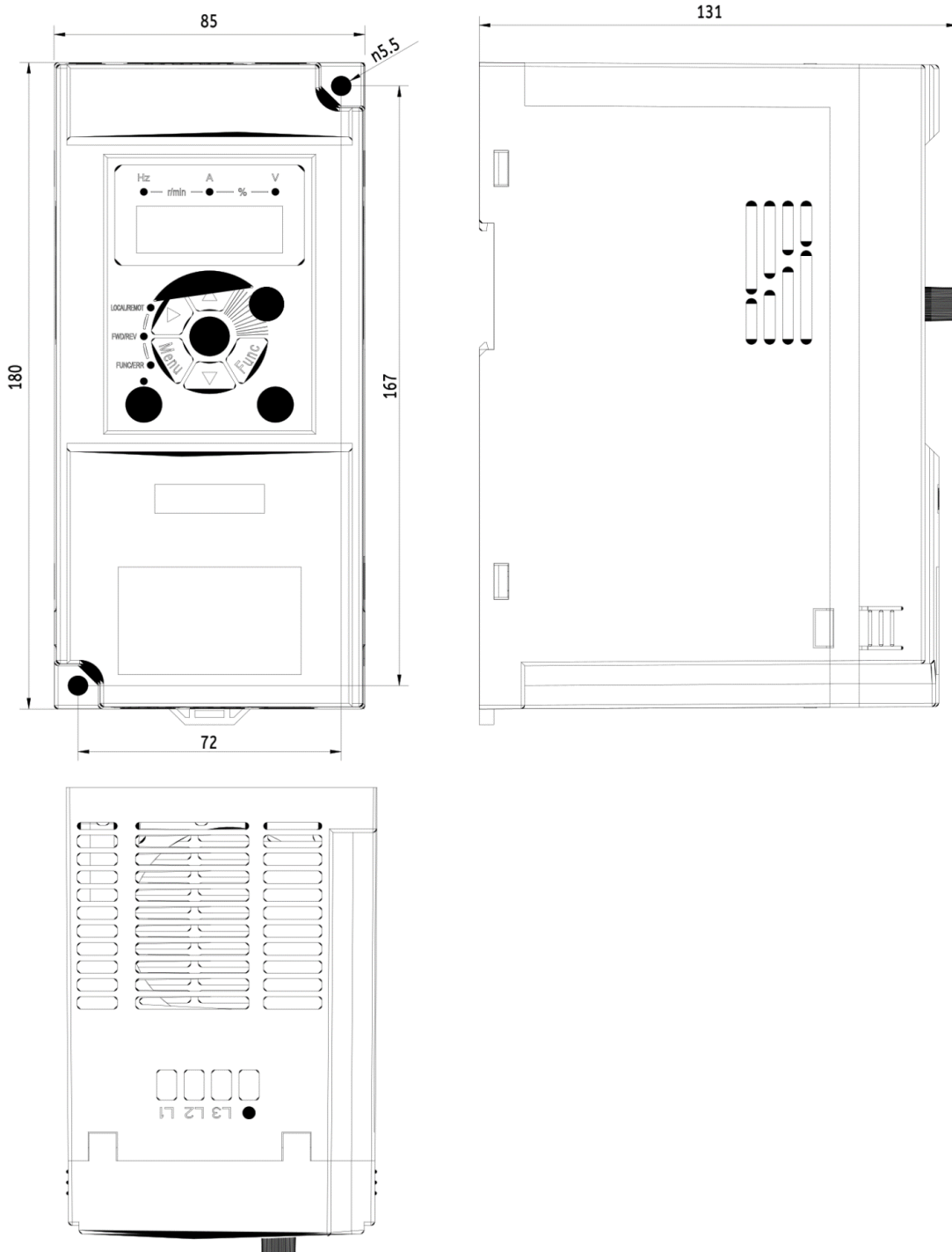
Dimensional drawing V900 - 4kW 4T0040
